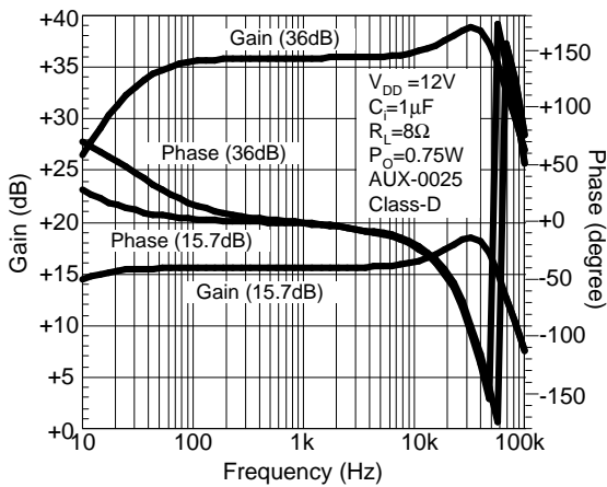
Frequency Response
